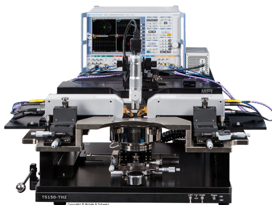
Fig. 2: The MPI TS150-THZ integrated probe system configured for measurement up to 330 GHz frequencies with the Rohde & Schwarz ZVA vector network analyzer. Picture is courtesy of Rohde and Schwarz.
