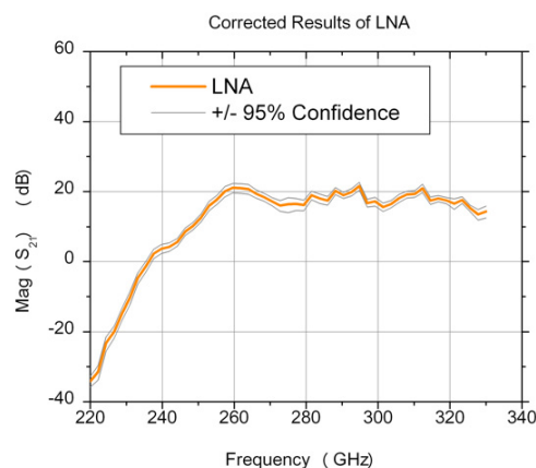
Fig. 15: The measured S21-parameter of the test MMIC measured with the respect to the multiline TRL including \pm 95\% confidence interval.
