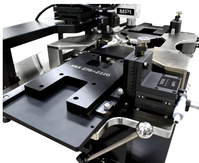
Fig. 4: The dove-tail interface of R&S®ZVA-Z75 to R&S®ZVA-Z220 frequency converters of the Rohde & Schwarz ZVA.
