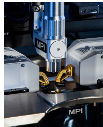
Fig. 3: The waveguide probes directly mounted at the output of the mm-wave VNA converters. Picture is courtesy of Rohde & Schwarz.
