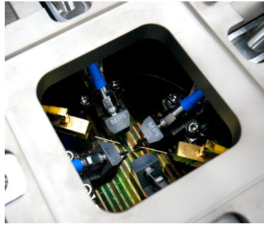
Typical MPI configuration with Kelvin Probes
